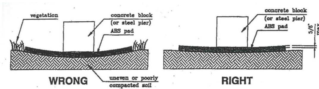
Figure 7. Maximum allowable deflection in a single ABS pad
